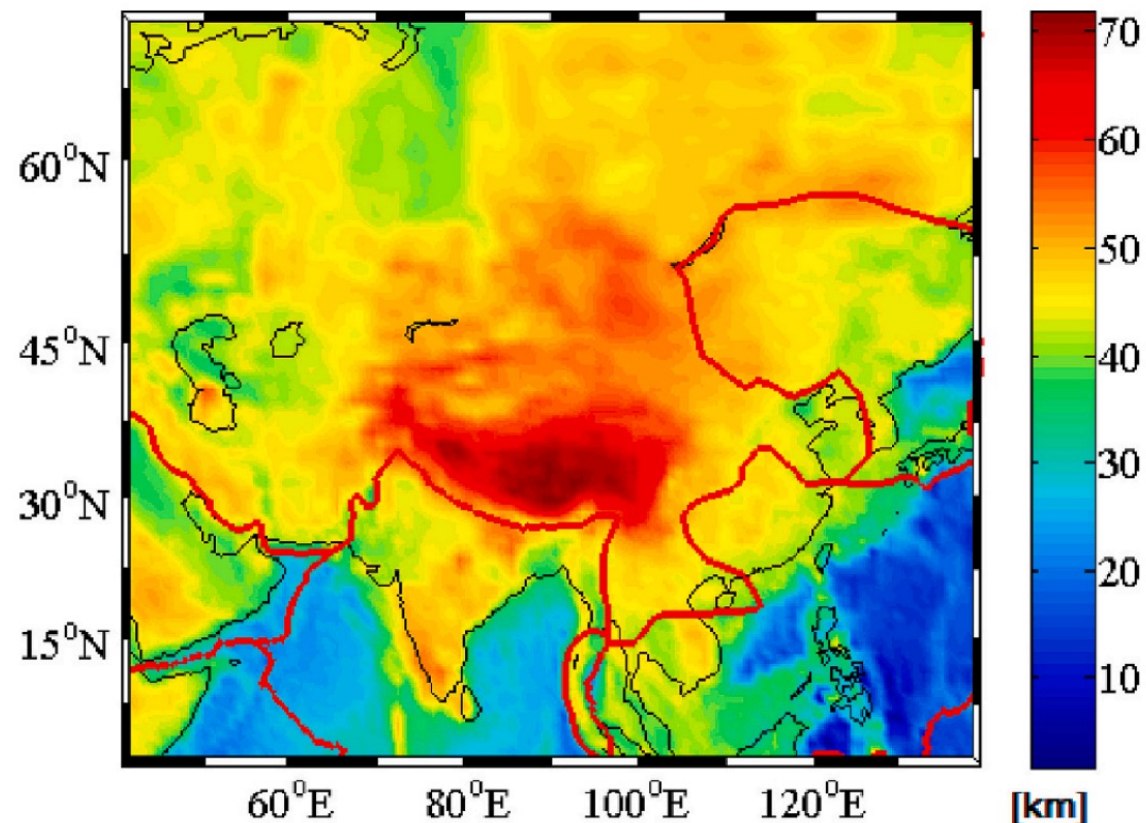
Map of the Moho depth computed from inversion of GOCE gravity gradients over Central Asia.
